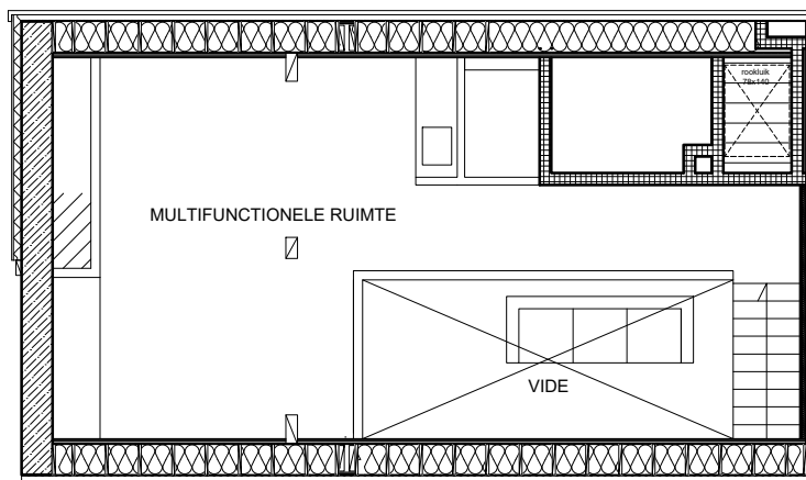
ZOLDERVERDIEPING
